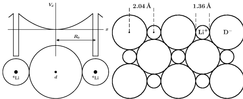
Fig. 12 Potential energy of a Deuteron nucleus with two neighboring Lithium atoms in a LiD crystal.
