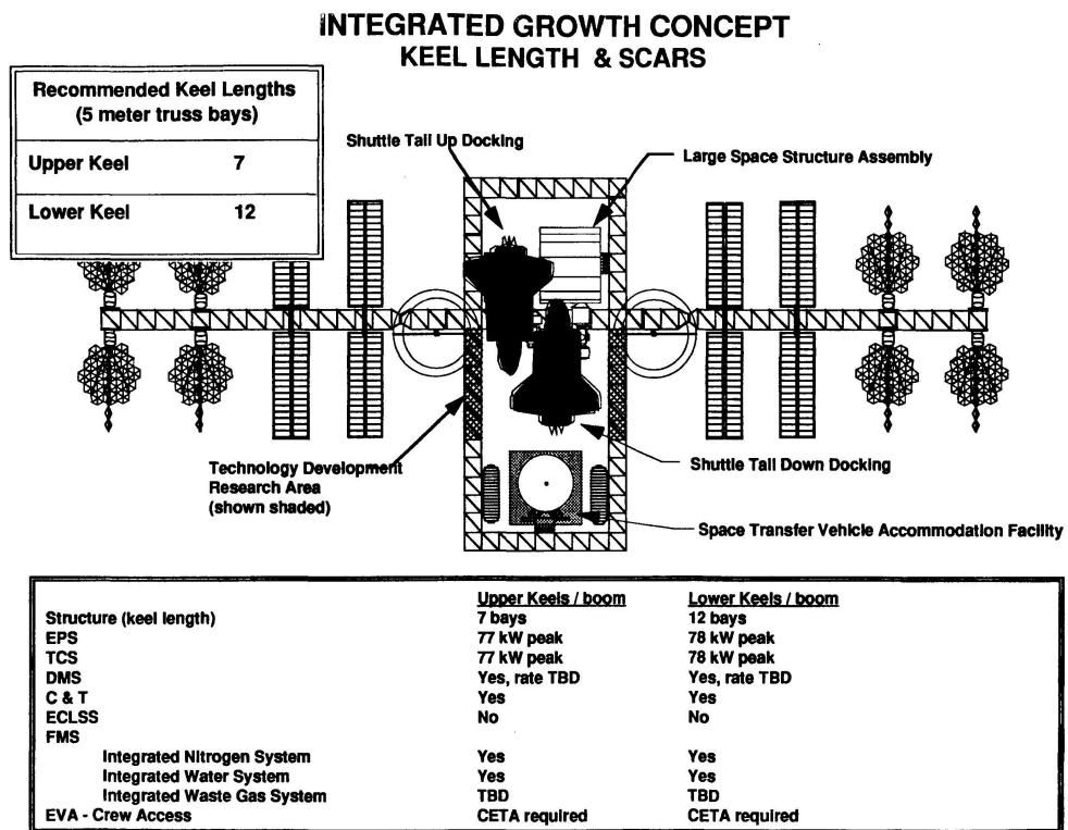
Fig. 14 Diagram from "Space Station Evolution - Beyond the Baseline" (Feb. 6 - 8, 1990, League City, Texas).
