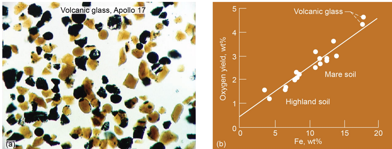
Fig. 5 Volcanic glass beads and oxygen yields from full range of Apollo samples.
