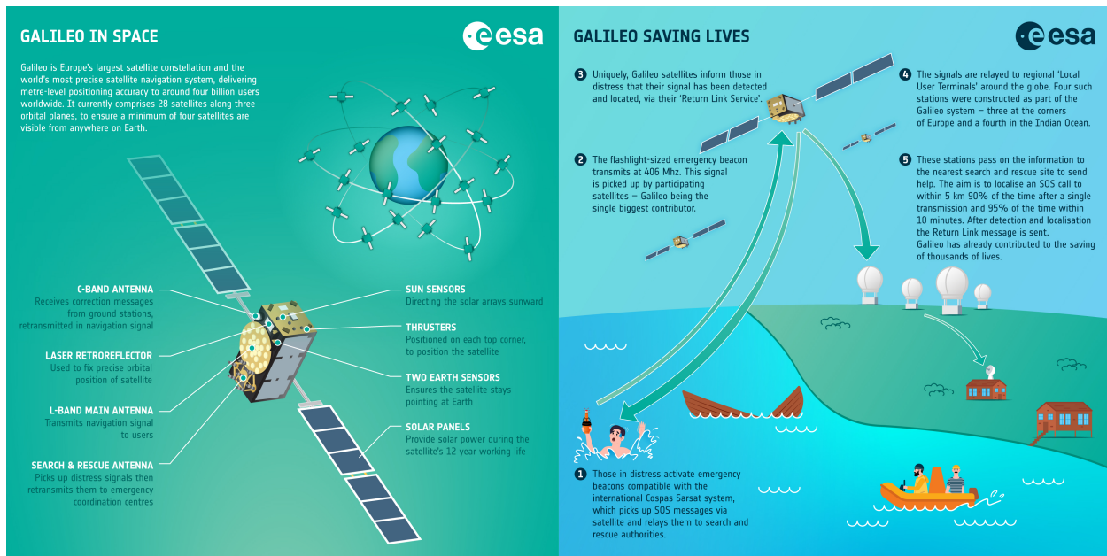
Fig. 6 Galileo is Europe’s largest satellite constellation and the world’s most precise satellite navigation system, delivering metre-level positioning accuracy to around four billion users worldwide. It currently comprises 28 satellites along three orbital planes, to ensure a minimum of four satellites are visible from anywhere on Earth.
