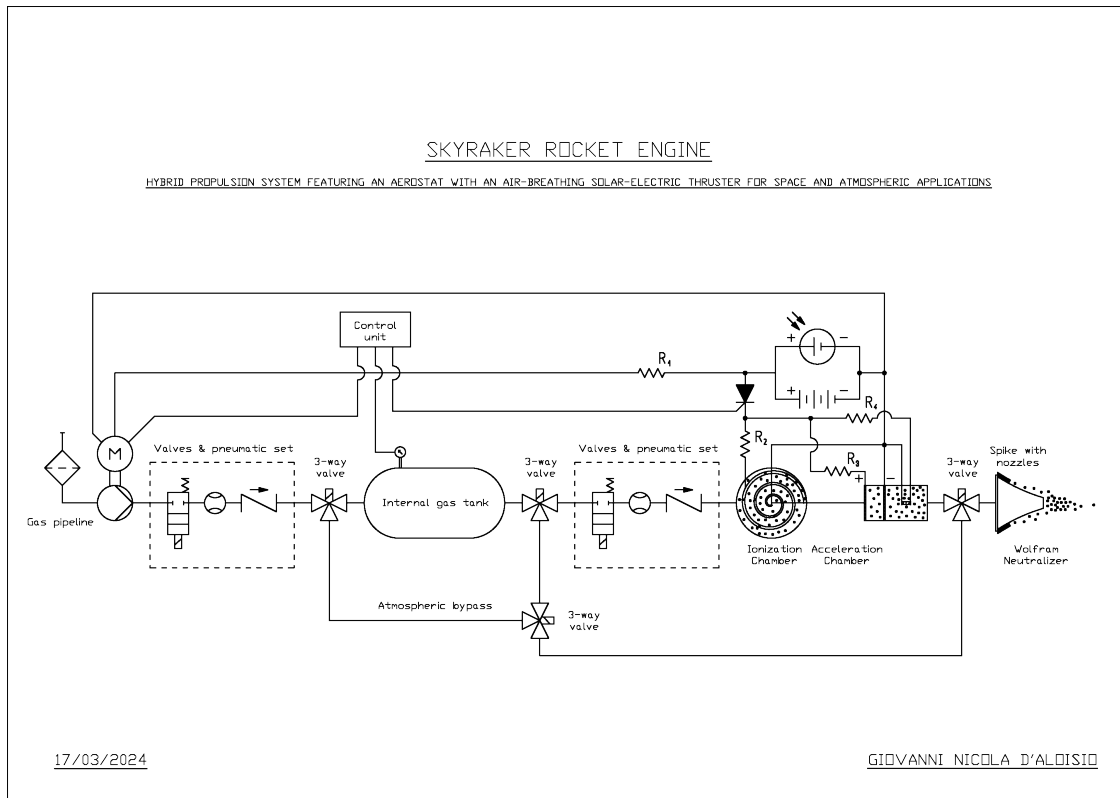
Fig. 11 Schematic flow diagram of a Skyraker rocket engine prototype.
