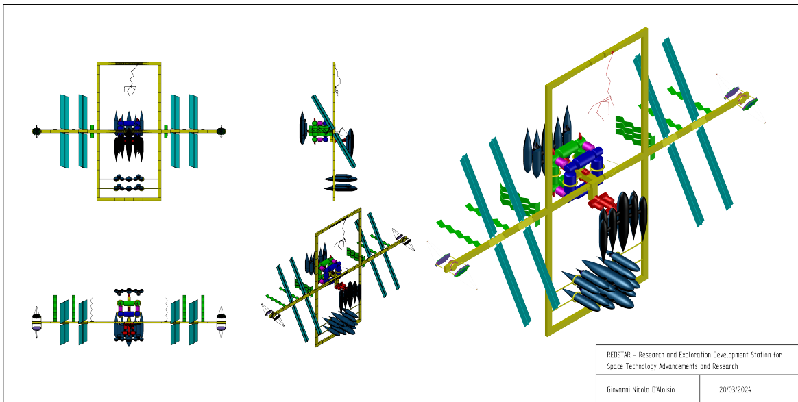
Fig. 13 Preliminary design of REDSTAR. Notice the INNOVATE and LUXE sections, behind the yellow Integrated Truss Structure, and the INFRAS section, red, in front of it. The huge black and blue vehicles are the Spectre S spacecrafts, docked at the station and at the shipyard. On the sides of the solar panels, there are the main communication antennas and the thermal radiators.
