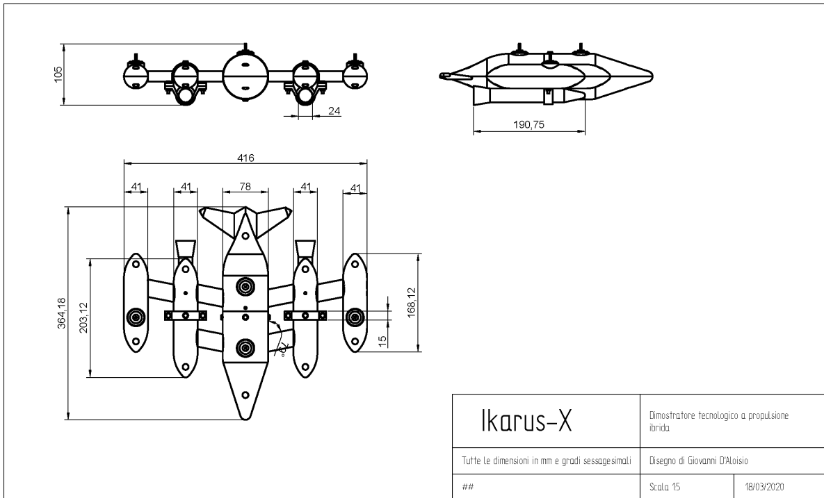
Fig. 9 Ikarus-X, the first aircraft of the Project Ikarus series.
